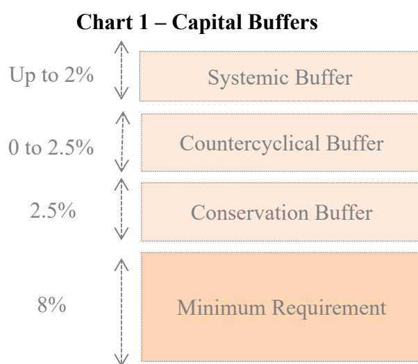
Description of regulatory capital requirements in Brazil, including the capital buffers: capital conservation buffer (CCoB), countercyclical capital buffer (CCyB) and for domestic systemically important banks (D-SIBs). See: https://www.bcb.gov.br/estabilidadefinanceira/regulacao_prudencial_normas
