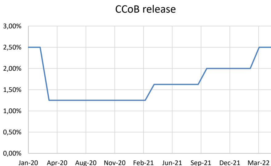
Chart 2 – CCoB release and gradual phase-out recovery
